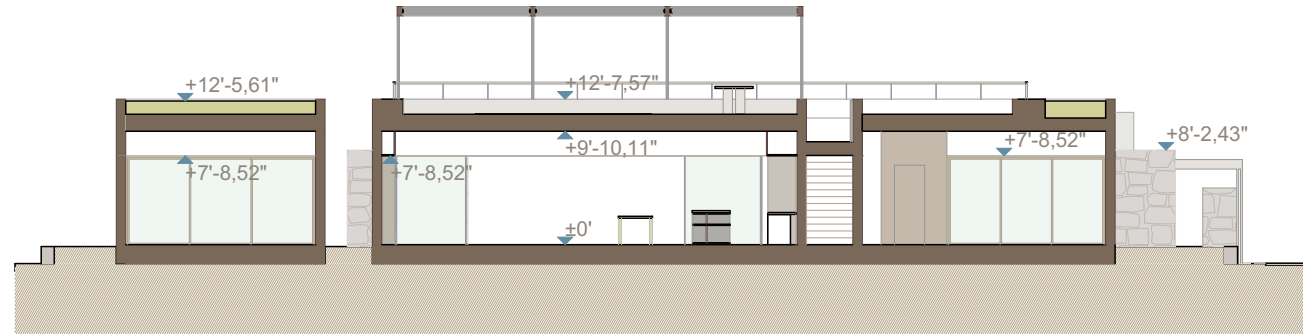
S-01 SECTION
